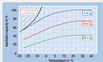
Available capacity as a function of temperature and discharge current.
